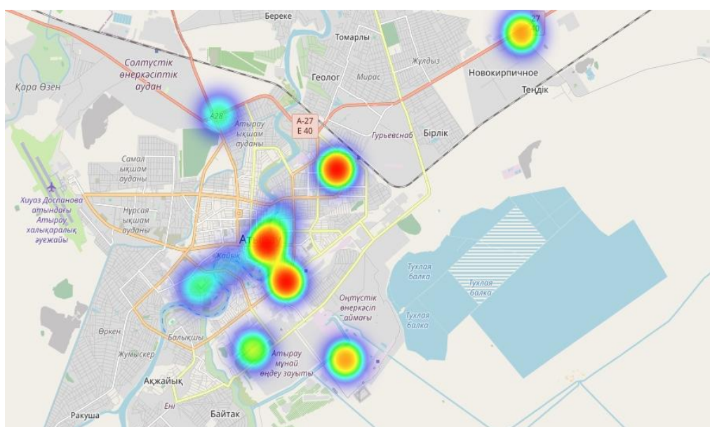
Figure 2. Heat Map of pollution October 2, 2024
