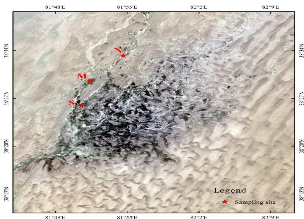
Fig. 1. Geographic location of the terminal area of the Keriya River and the distribution of sampling sites. The labels S, M, and N represent sampling sites in the southern, middle, and northern parts of the study area, respectively.
