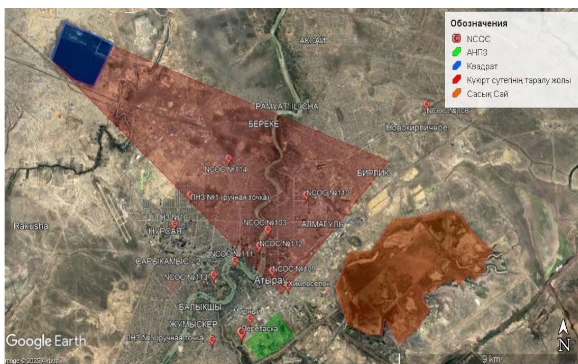
Figure 4. map of the distribution of hydrogen sulfide in Atyrau October 9, 2024
