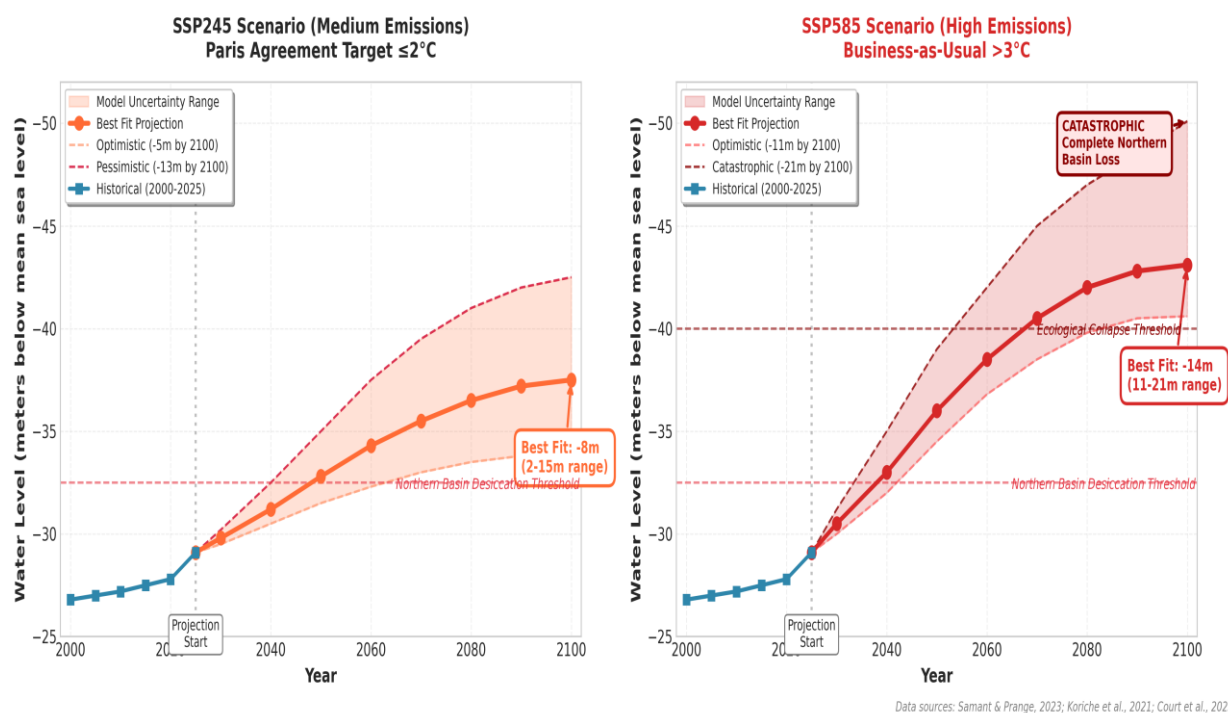
Figure 2. Projected Caspian Sea level decline scenarios to 2100
