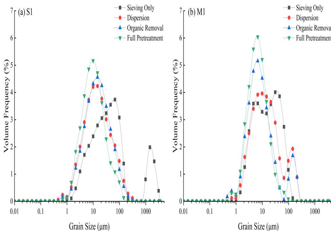
Fig. 2. Grain-size frequency distribution curves of fluvial sediments in desert regions under stepwise pretreatment conditions
