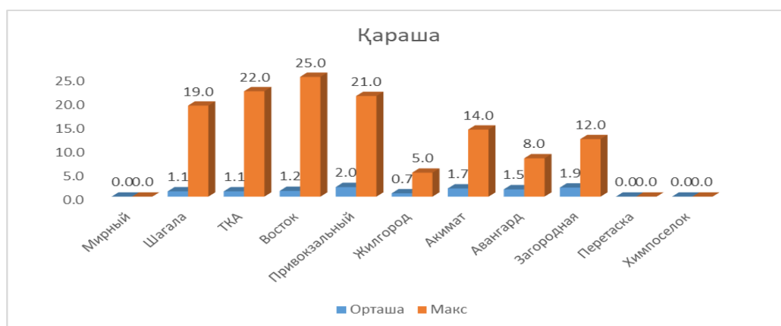
Figure 5. dynamics of hydrogen sulfide concentration in environmental posts in November 2024.
