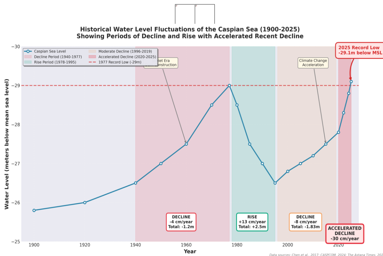
Figure 1. Historical water level fluctuations of the Caspian Sea (1900-2025)
