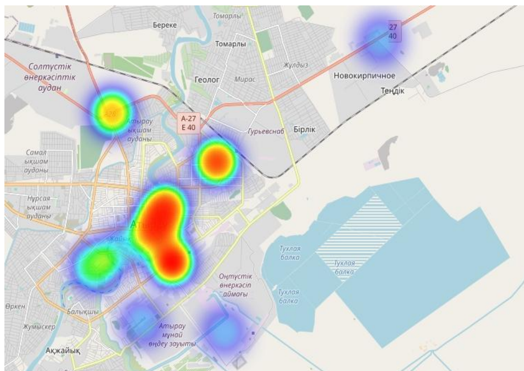
Figure 3. The figure shows a thermal map reflecting the spatial distribution of hydrogen sulfide concentration in Atyrau on the night of October 6-7, 2024
