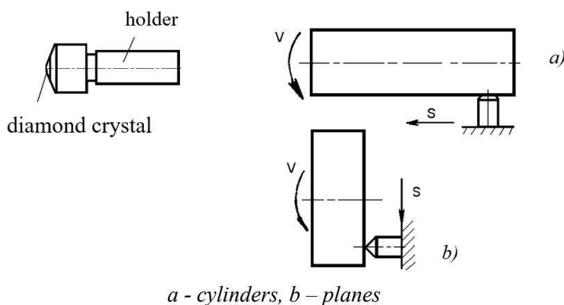
Figure 1 - Diamond ironing machine and ironing schemes
