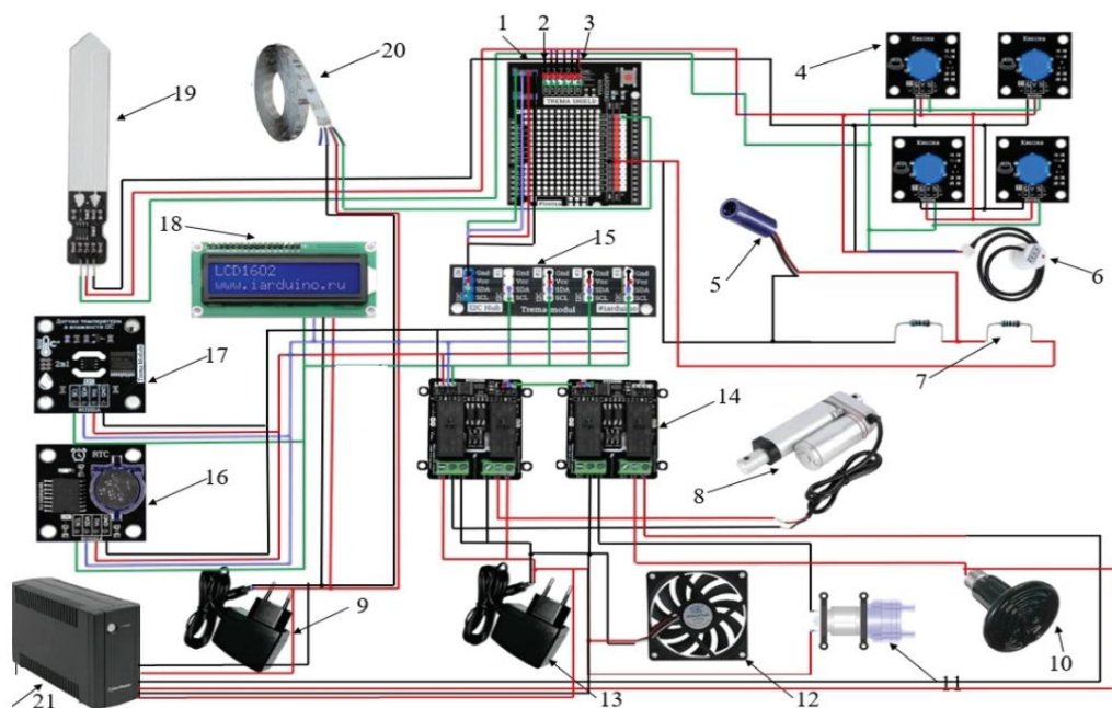
Figure 5 – Connection diagram of the laboratory complex components
