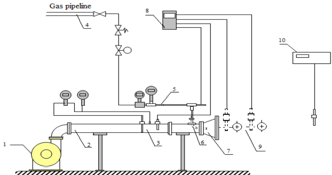
Figure 2-Experimental stand
