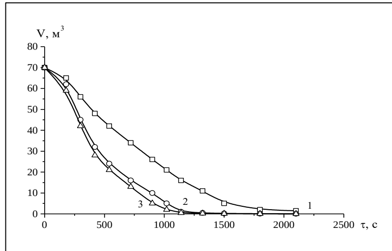
Figure 1 – Change in the estimated volume of oil mixtures from the Zhetybay, Uzen, Kalamkas, and Karazhanbas fields in a tank depending on the draining time. 1 - initial oil mixture, the ratio of oils is: Zhetybay-Uzen - 65%, Karazhanbas-Kalamkas - 35%; 2 - the same oil after cavitation treatment, \tau = 10 minutes; 3 - the same oil after cavitation treatment, \tau = 15 minutes. System temperature is 30°C
