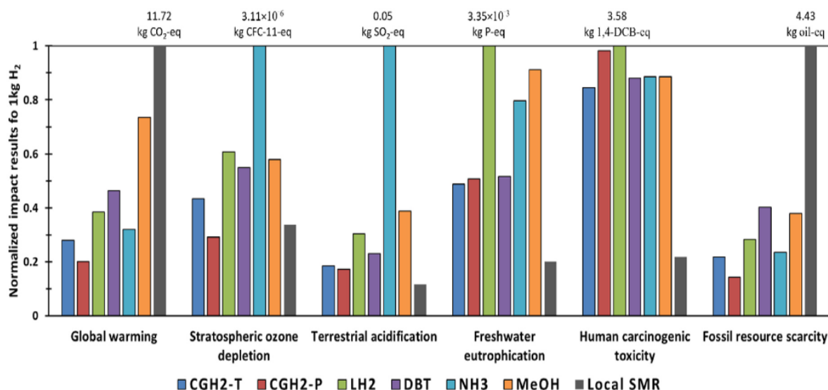
Figure 2. Environmental impact comparison of six green H 2 delivery scenarios of 1 kg of H 2 [15]
